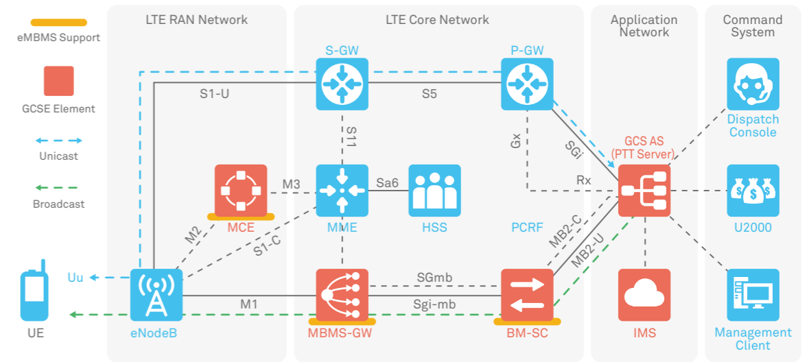
Figure 11 Optional Architecture of LTE Trunking Solution
