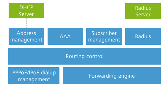
Figure 3-1 BNG architecture for traditional metro networks
