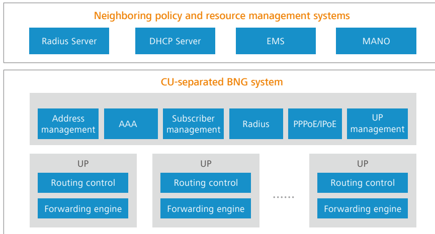
Figure 3-2 Logical architecture of a C/U separated BNG
