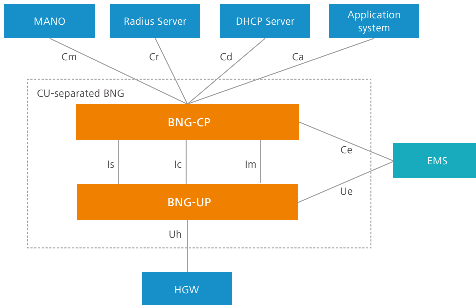
Figure 3-3 System interfaces
