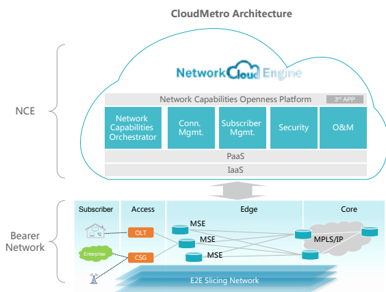
Figure 4-1 CloudMetro architecture
